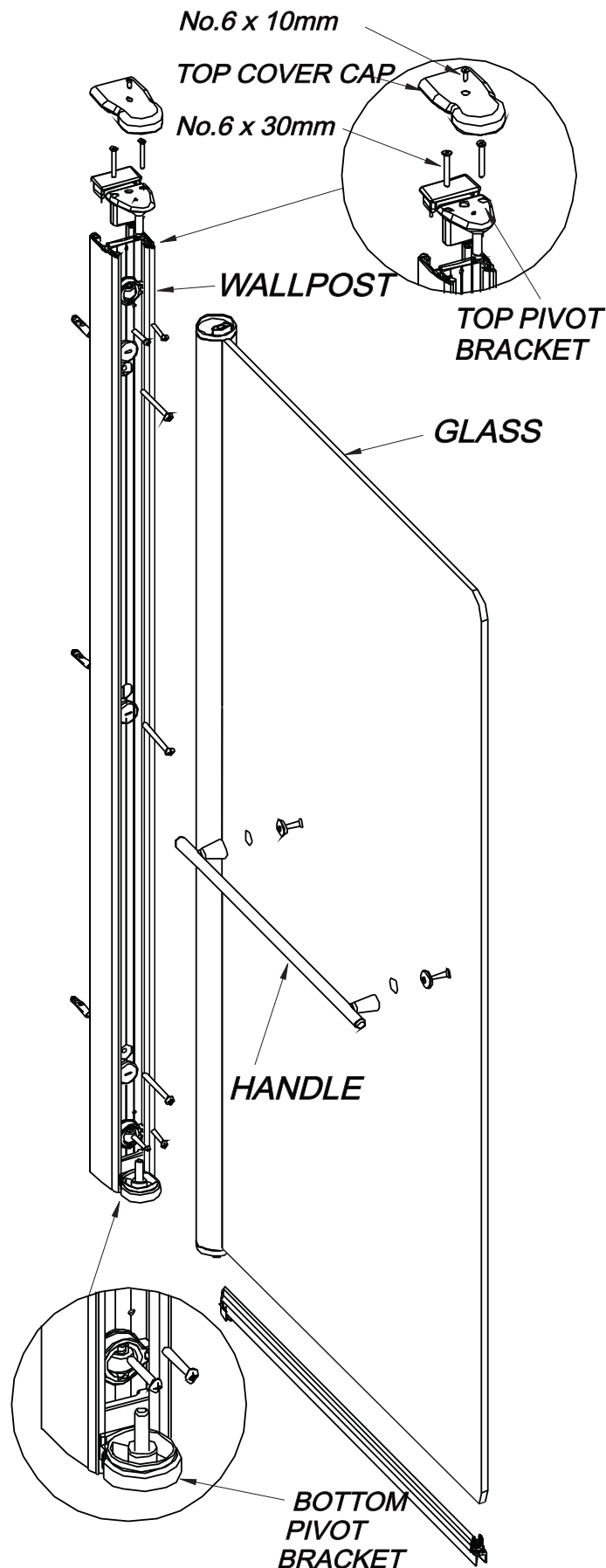
BATHSCREEN - EXPLODED VIEW
