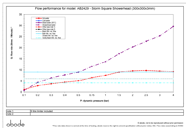
Storm Slimline 300mm Square Showerhead AB2429 v2 © abode home products ltd www.abode.eu our policy is to continually improve our product quality, and accordingly we reserve the right to amend specifications without prior notice
