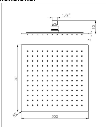
Storm Slimline 300mm Square Showerhead AB2429 v2 © abode home products ltd www.abode.eu our policy is to continually improve our product quality, and accordingly we reserve the right to amend specifications without prior notice
