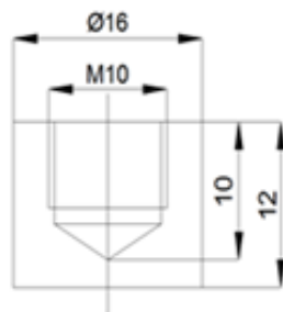
BRACKET PIN Ø16
