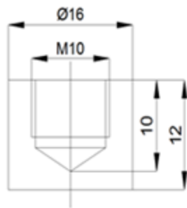
BRACKET PIN Ø16
