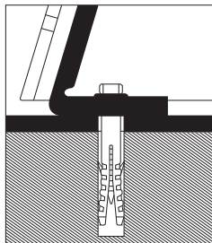
Put on the new WC Pan
